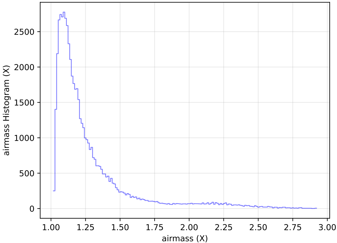
ddf_loaded_fl8_v3.4_10yrs Yr 1 i band: airmass Histogram
