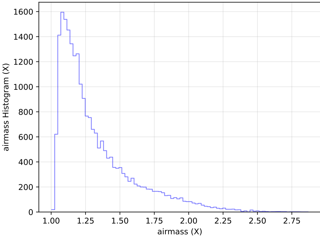
ddf_loaded_fl8_v3.4_10yrs Yr 1 g band: airmass Histogram
