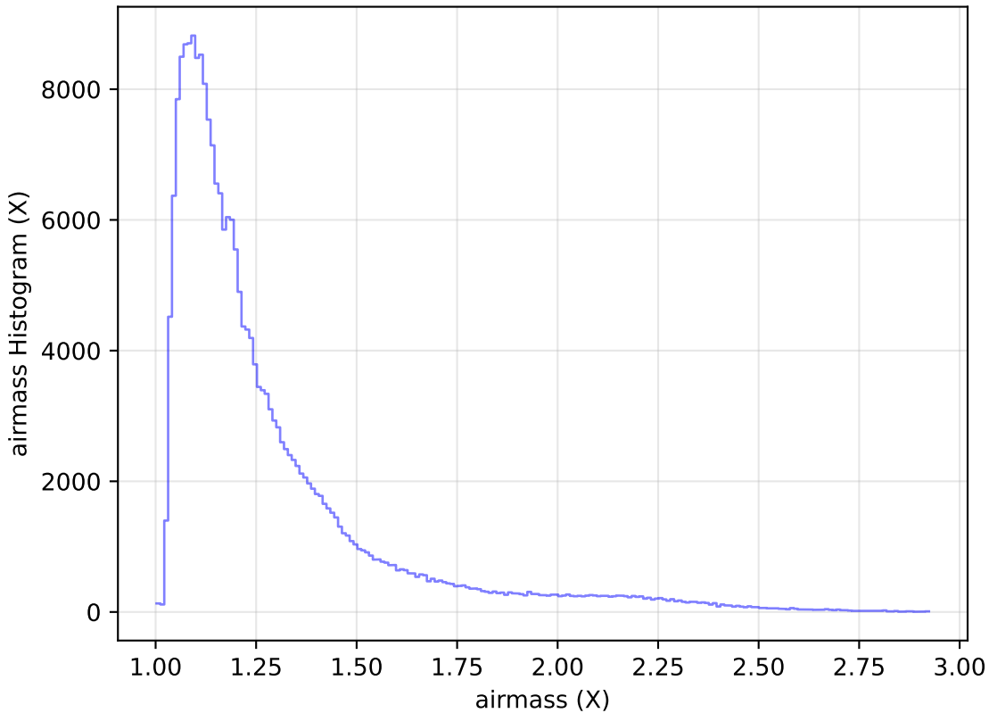
ddf_loaded_fl8_v3.4_10yrs Yr 1 all bands: airmass Histogram
