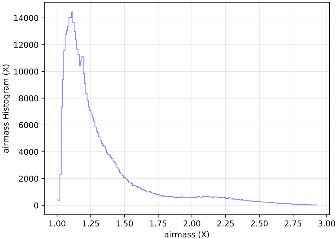
ddf_loaded_fl8_v3.4_10yrs WFD z band: airmass Histogram
