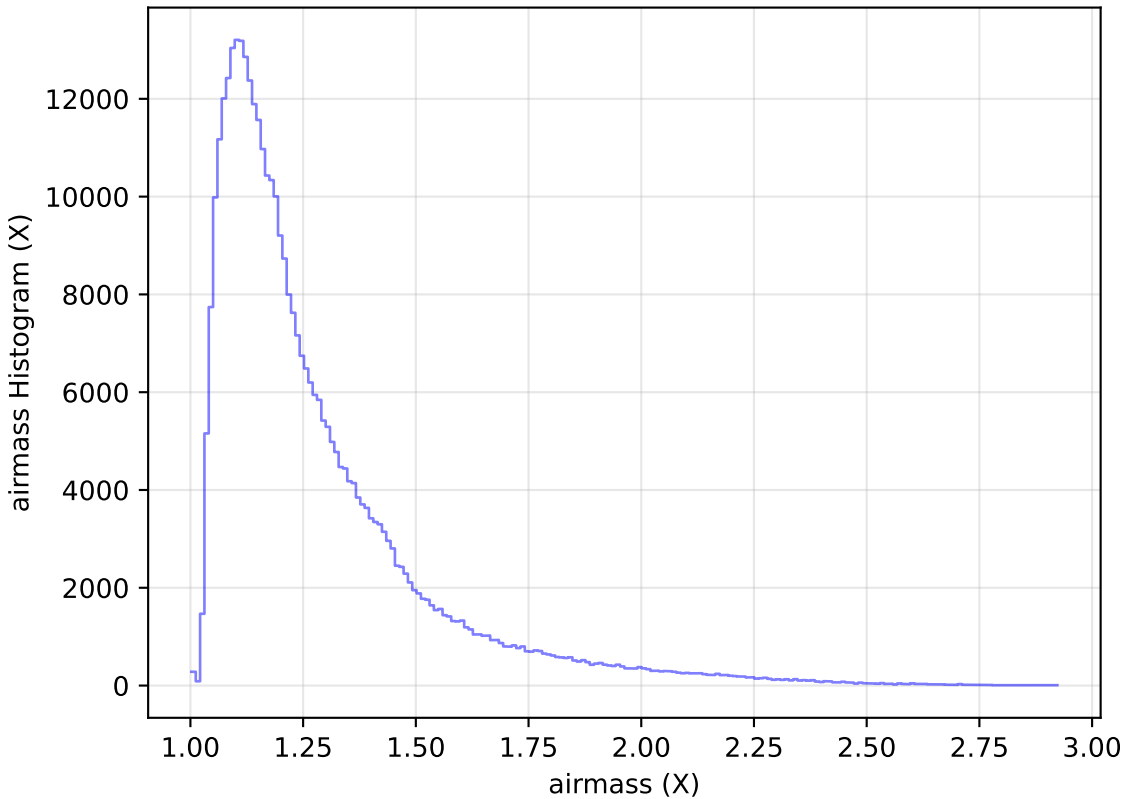
ddf_loaded_fl8_v3.4_10yrs WFD y band: airmass Histogram
