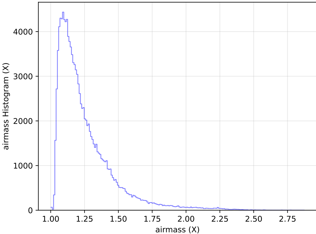
ddf_loaded_fl8_v3.4_10yrs WFD u band: airmass Histogram
