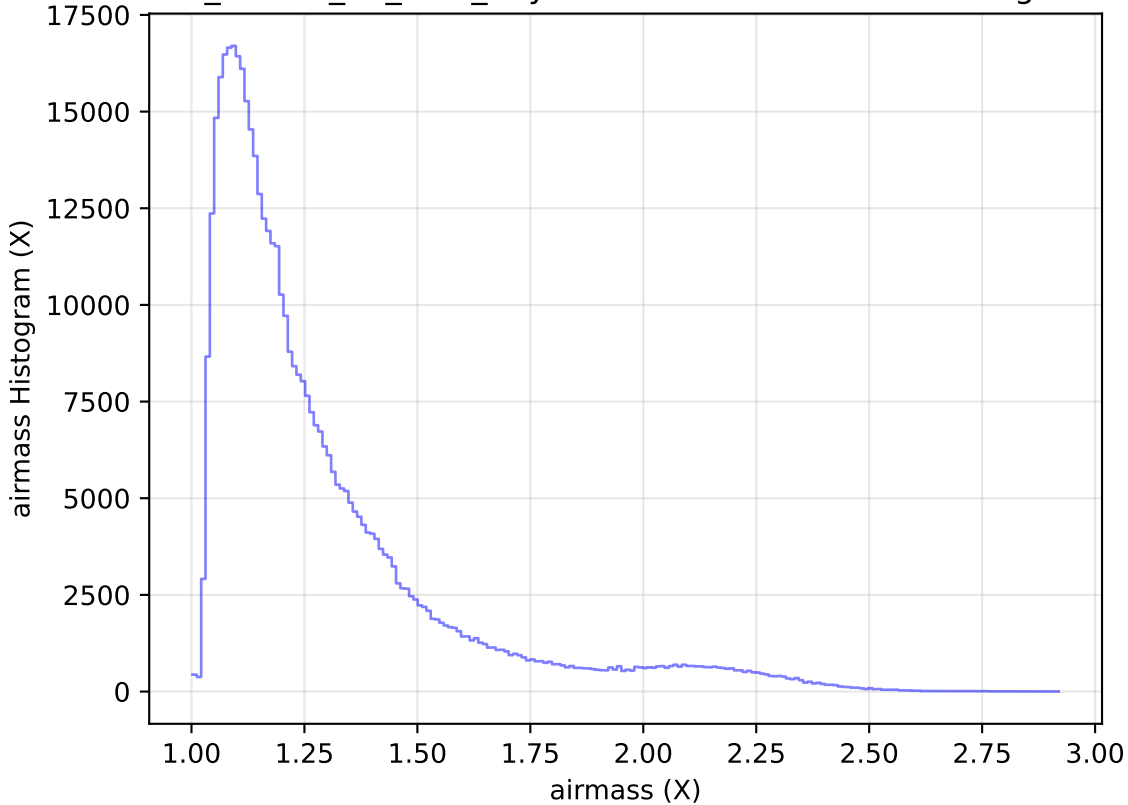
ddf_loaded_fl8_v3.4_10yrs WFD r band: airmass Histogram
