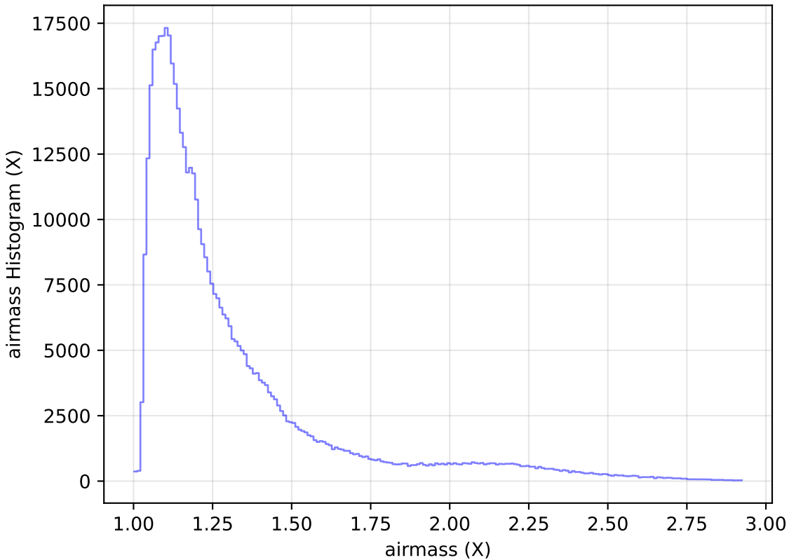
ddf_loaded_fl8_v3.4_10yrs WFD i band: airmass Histogram
