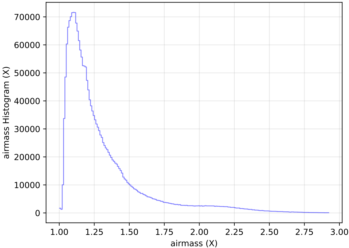
ddf_loaded_fl8_v3.4_10yrs WFD all bands: airmass Histogram
