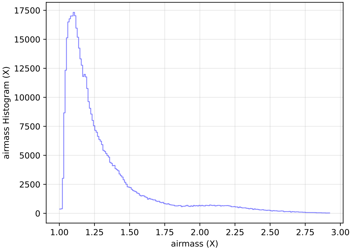
ddf_loaded_fl8_v3.4_10yrs All sky i band: airmass Histogram
