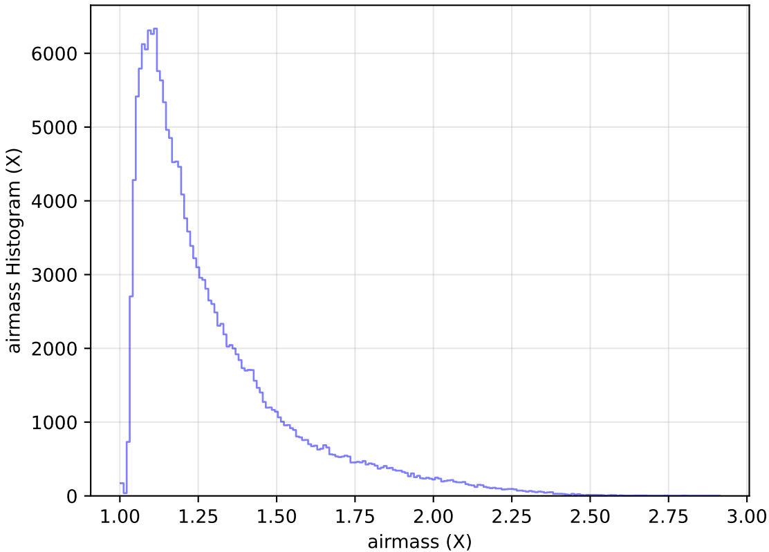
ddf_loaded_fl8_v3.4_10yrs All sky g band: airmass Histogram
