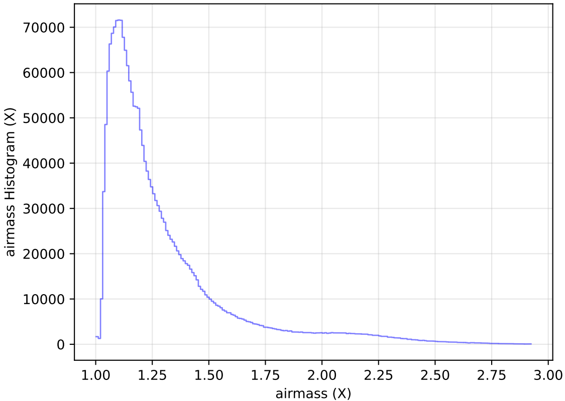
ddf_loaded_fl8_v3.4_10yrs All sky all bands: airmass Histogram
