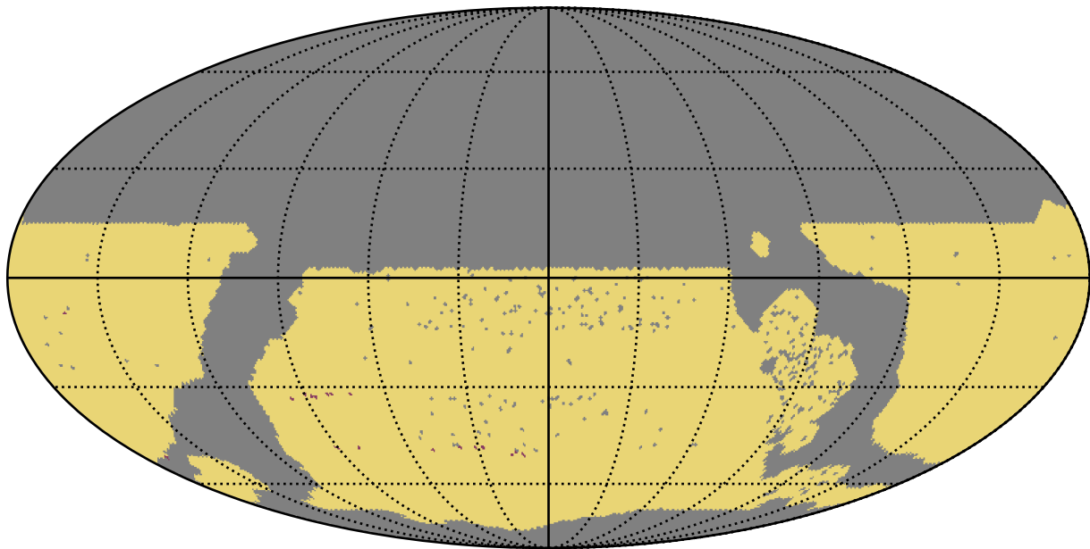
ddf_loaded_fl8_v3.4_10yrs WFD: RapidRevisits
