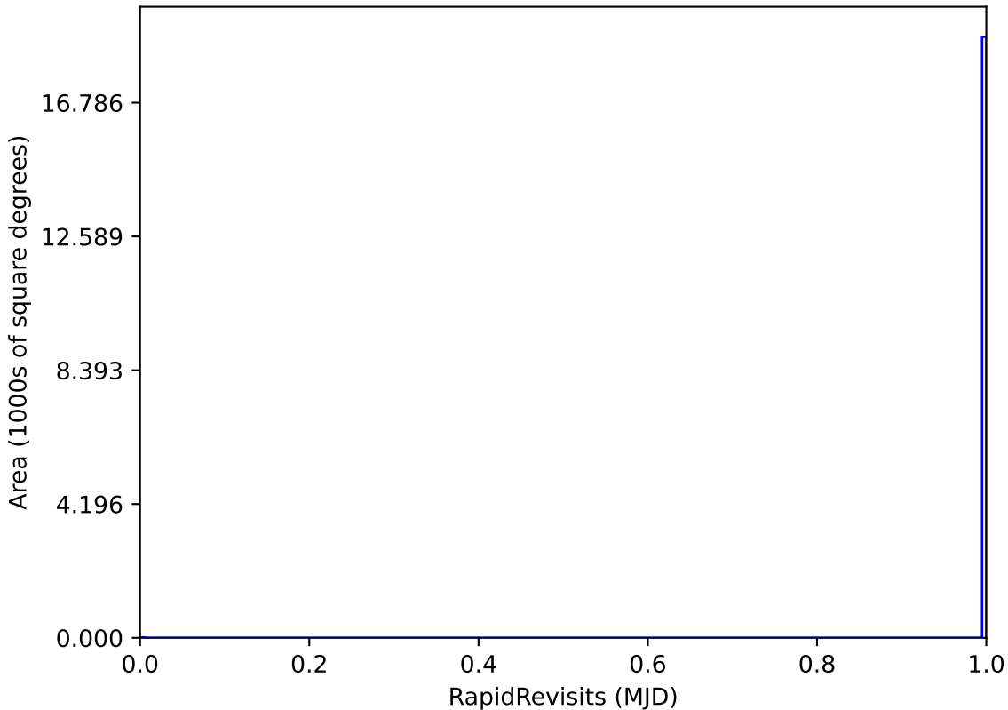
ddf_loaded_fl8_v3.4_10yrs WFD: RapidRevisits
