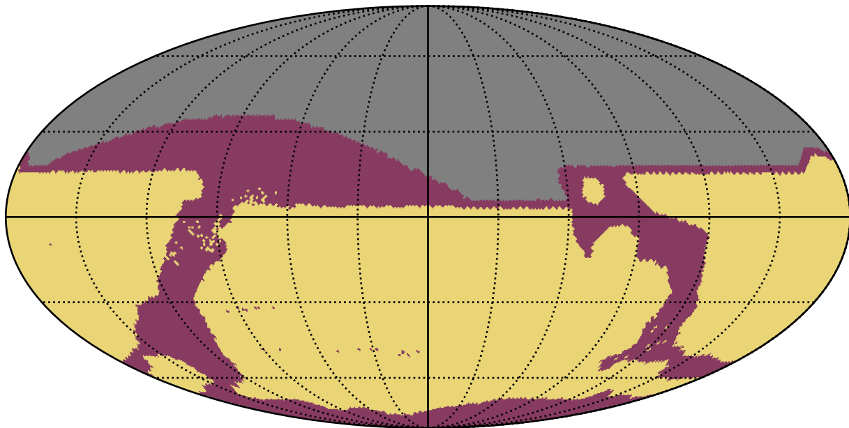
ddf_loaded_fl8_v3.4_10yrs All sky: RapidRevisits
