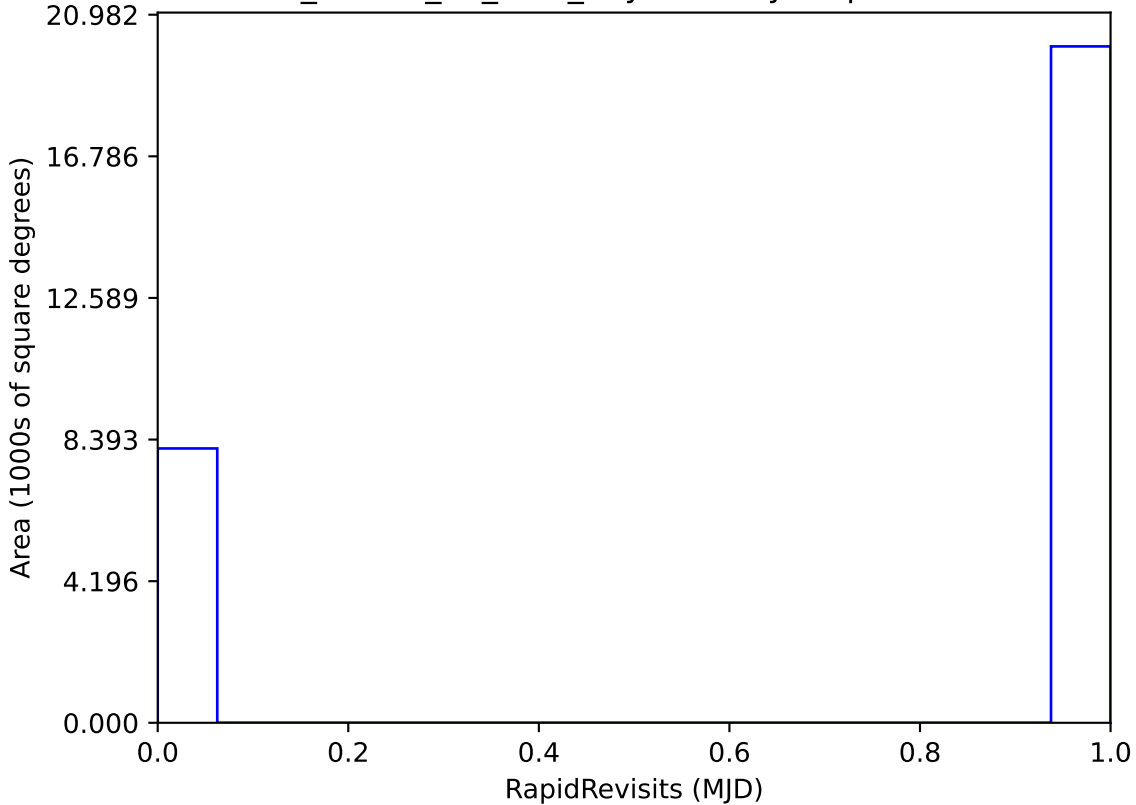
ddf_loaded_fl8_v3.4_10yrs All sky: RapidRevisits
