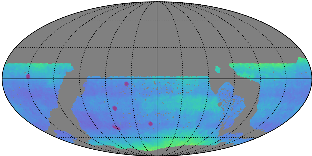
ddf_loaded_fl8_v3.4_10yrs WFD: Proper Motion Uncert @ 24.0
