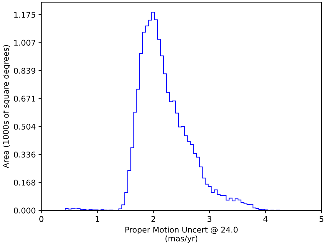
ddf_loaded_fl8_v3.4_10yrs WFD: Proper Motion Uncert @ 24.0
