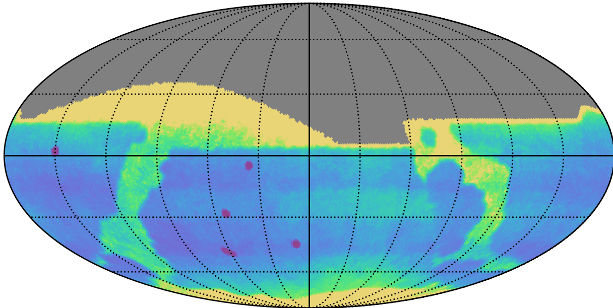
ddf_loaded_fl8_v3.4_10yrs All sky: Proper Motion Uncert @ 24.0
