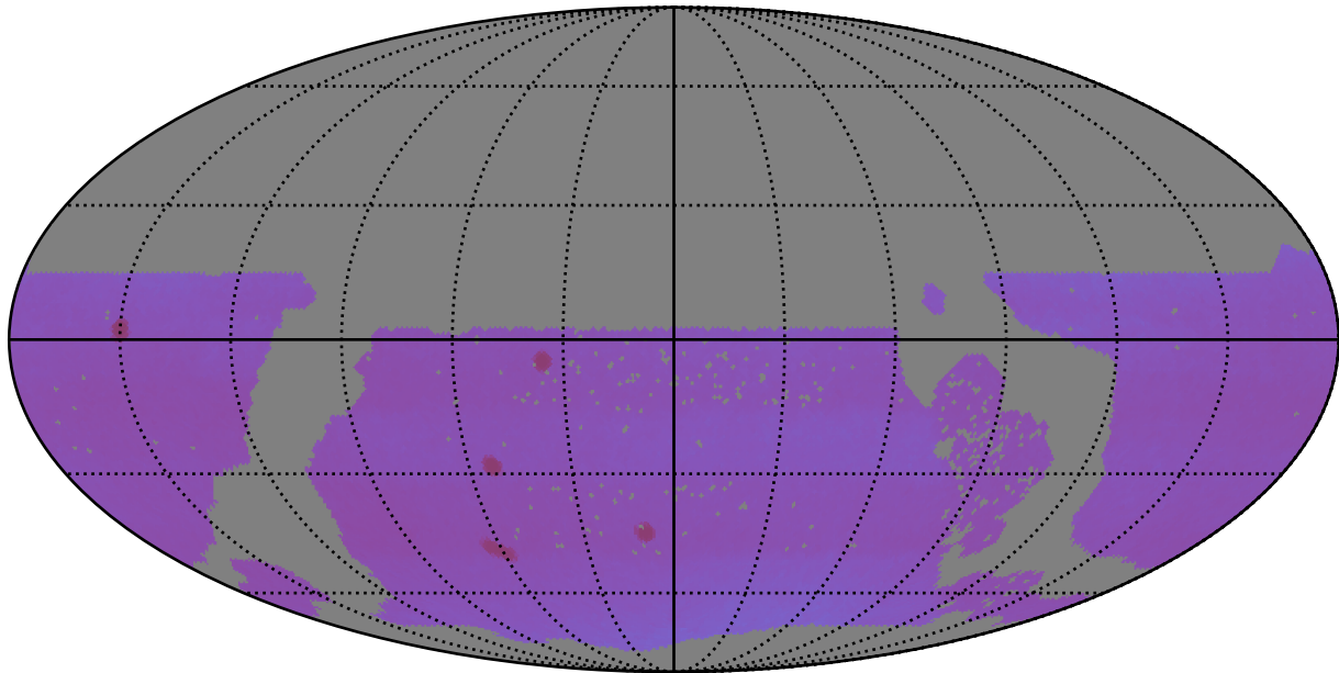
ddf_loaded_fl8_v3.4_10yrs WFD: Proper Motion Uncert @ 20.5
