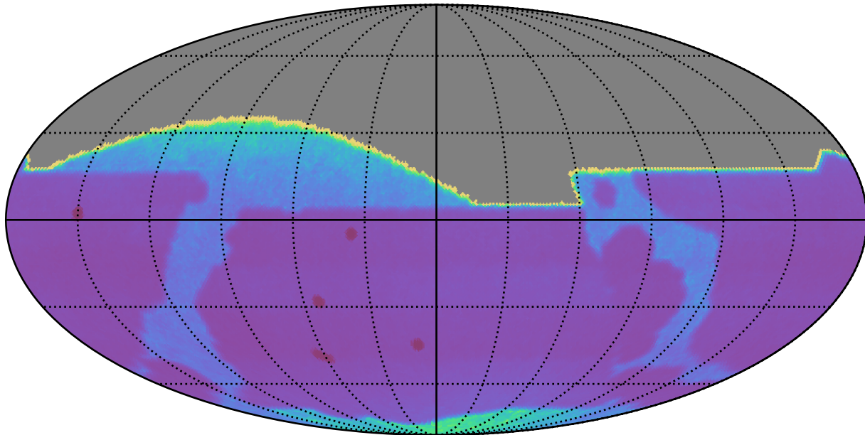
ddf_loaded_fl8_v3.4_10yrs All sky: Proper Motion Uncert @ 20.5
