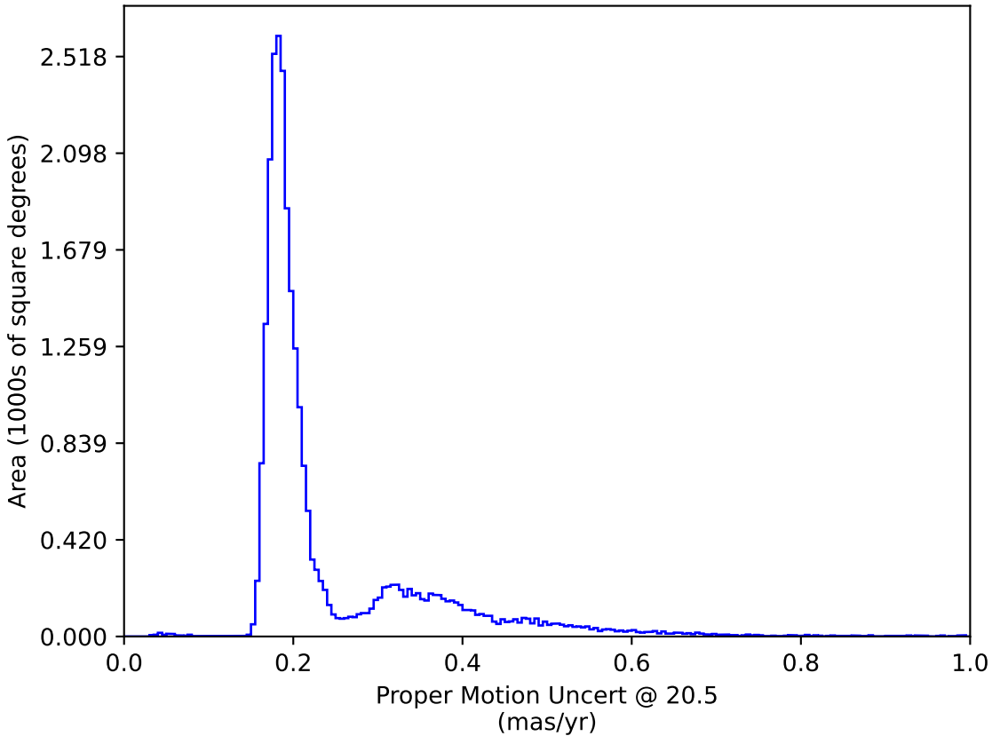
ddf_loaded_fl8_v3.4_10yrs All sky: Proper Motion Uncert @ 20.5
