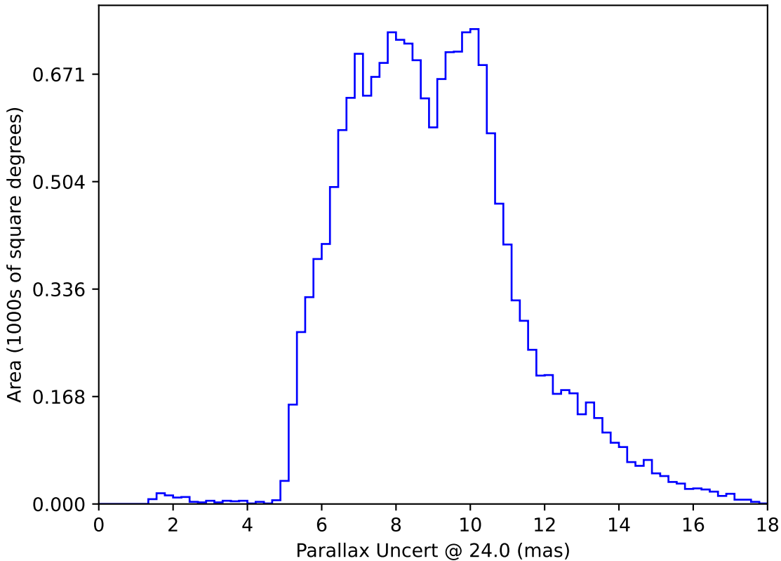
ddf_loaded_fl8_v3.4_10yrs WFD: Parallax Uncert @ 24.0
