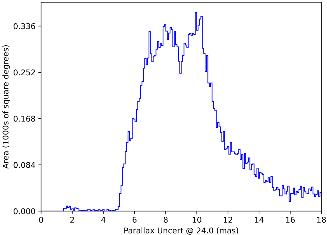
ddf_loaded_fl8_v3.4_10yrs All sky: Parallax Uncert @ 24.0
