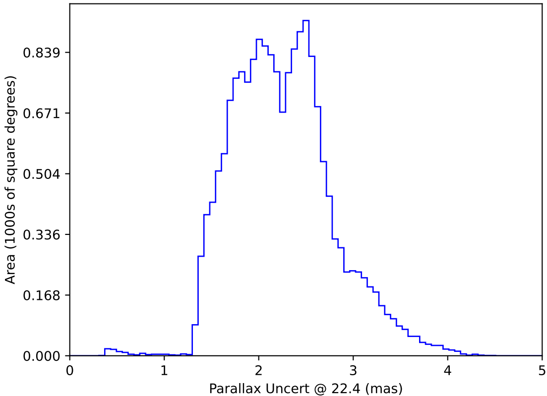
ddf_loaded_fl8_v3.4_10yrs WFD: Parallax Uncert @ 22.4
