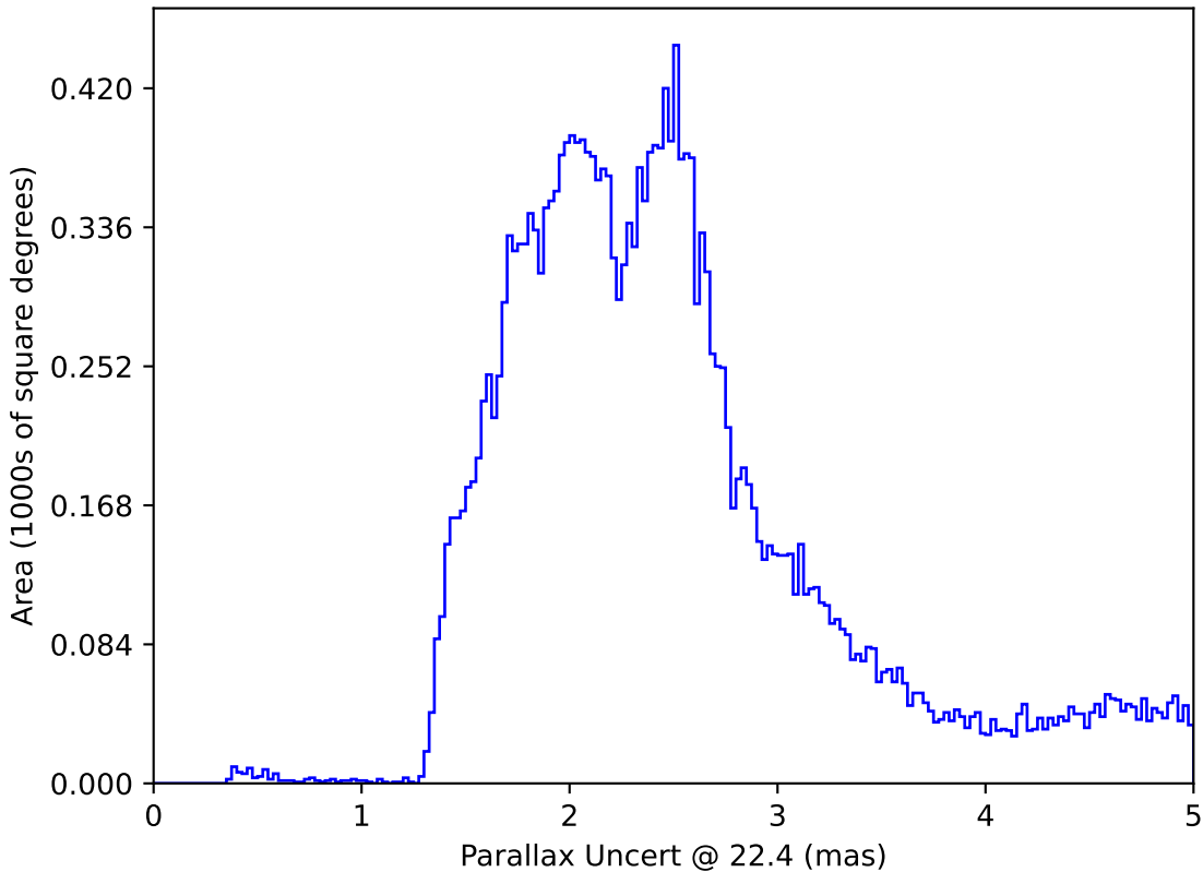
ddf_loaded_fl8_v3.4_10yrs All sky: Parallax Uncert @ 22.4
