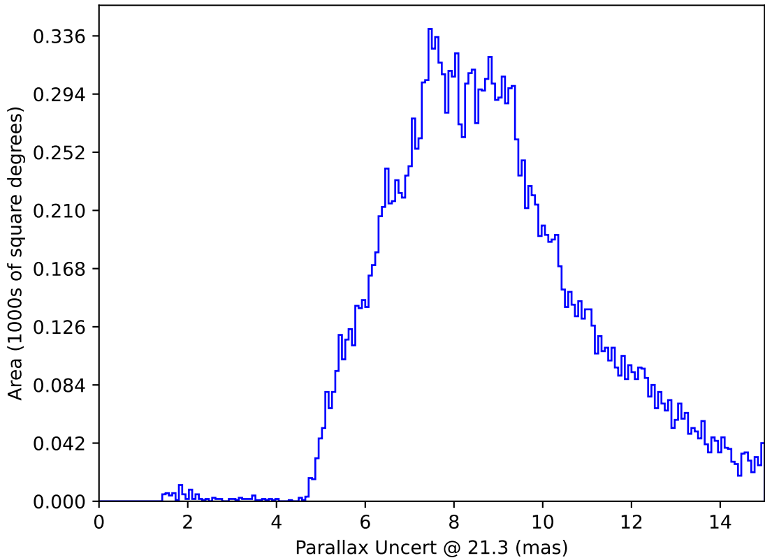
ddf_loaded_fl8_v3.4_10yrs All sky y band only: Parallax Uncert @ 21.3
