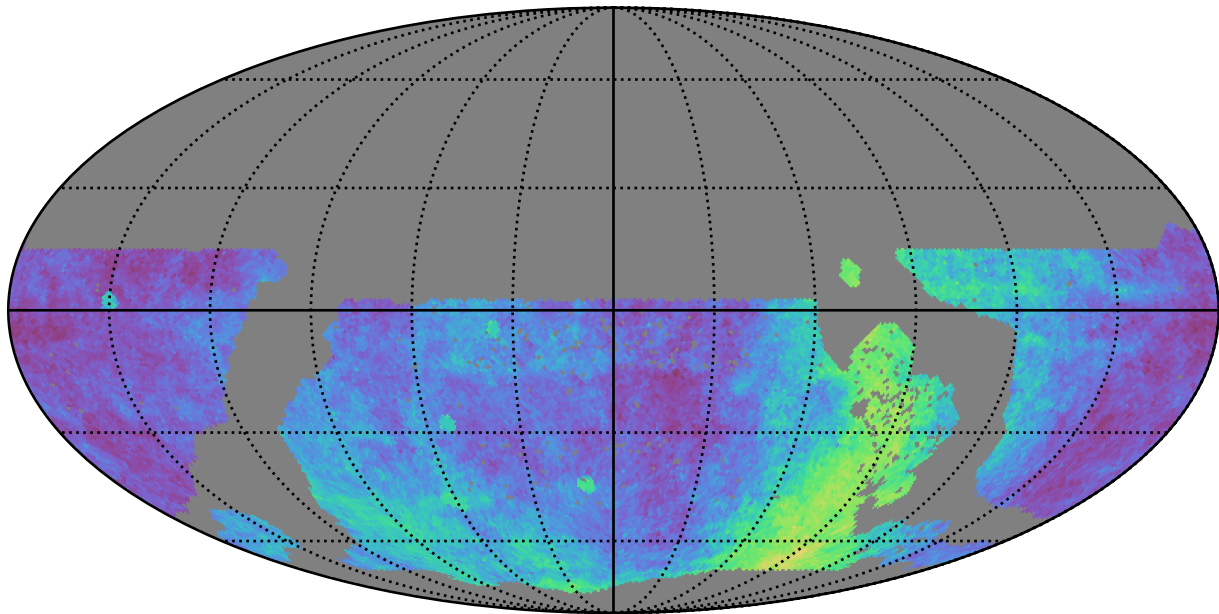
ddf_loaded_fl8_v3.4_10yrs WFD: Parallax Coverage @ 24.0
