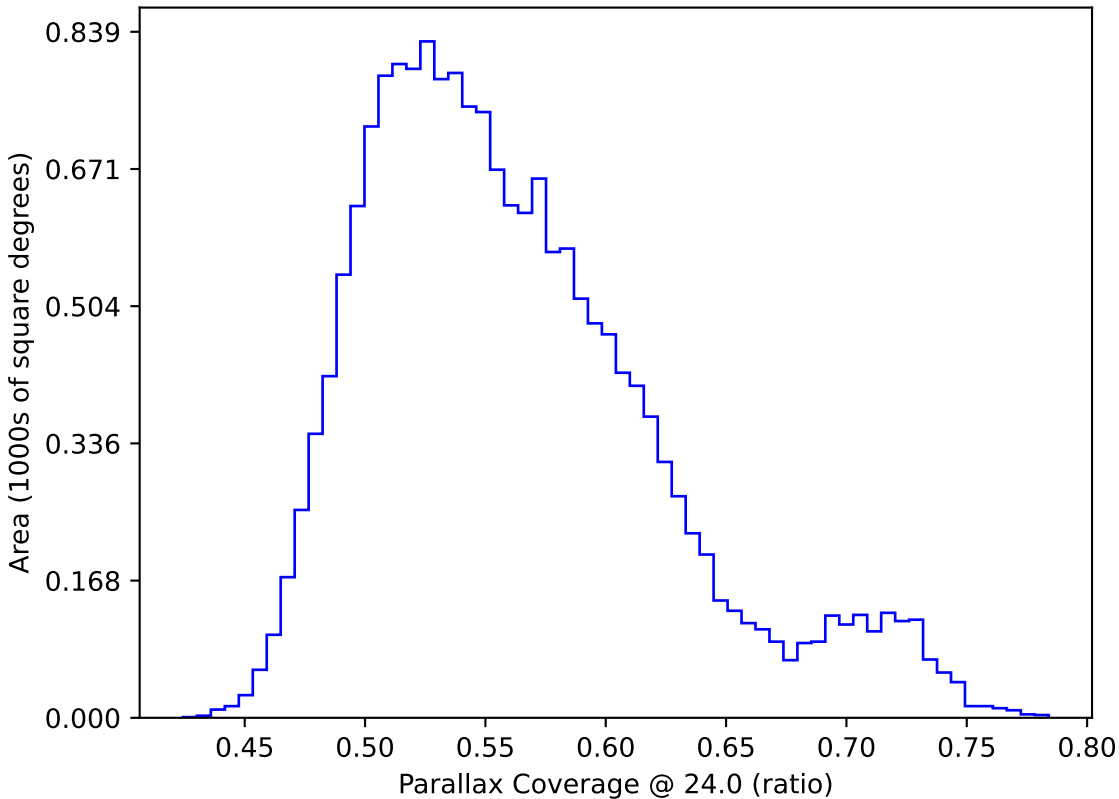
ddf_loaded_fl8_v3.4_10yrs WFD: Parallax Coverage @ 24.0
