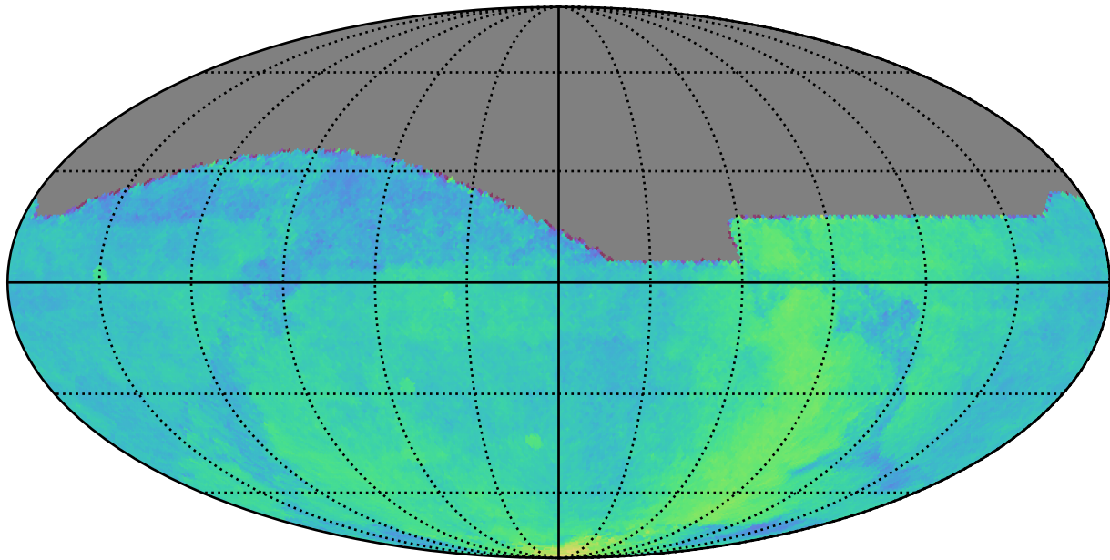
ddf_loaded_fl8_v3.4_10yrs All sky: Parallax Coverage @ 24.0
