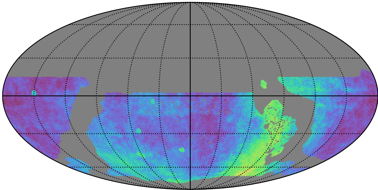
ddf_loaded_fl8_v3.4_10yrs WFD: Parallax Coverage @ 22.4
