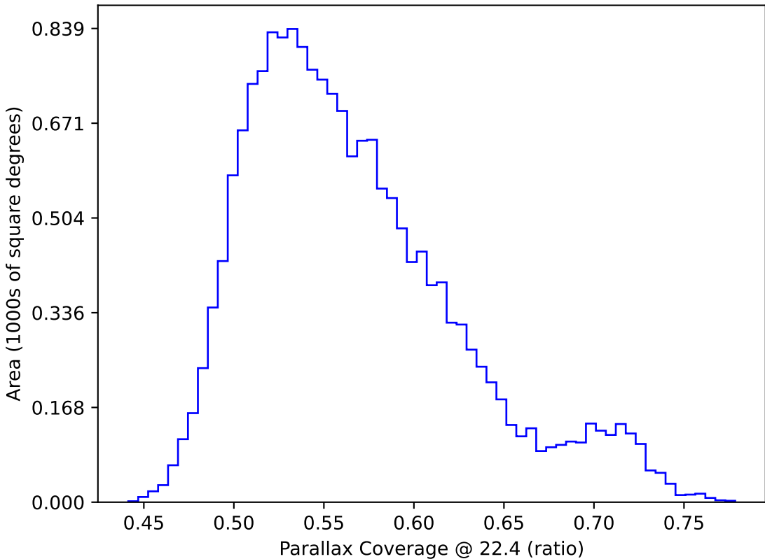
ddf_loaded_fl8_v3.4_10yrs WFD: Parallax Coverage @ 22.4
