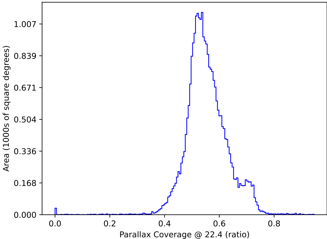
ddf_loaded_fl8_v3.4_10yrs All sky: Parallax Coverage @ 22.4
