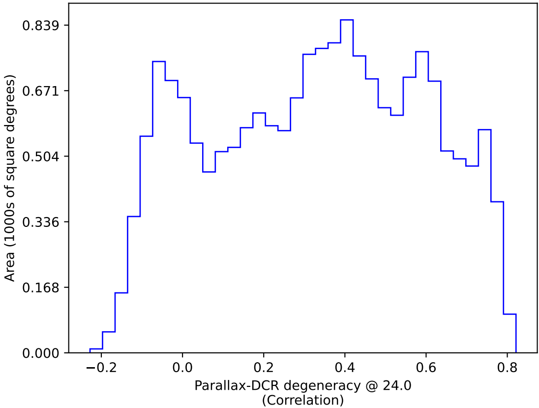
ddf_loaded_fl8_v3.4_10yrs WFD: Parallax-DCR degeneracy @ 24.0
