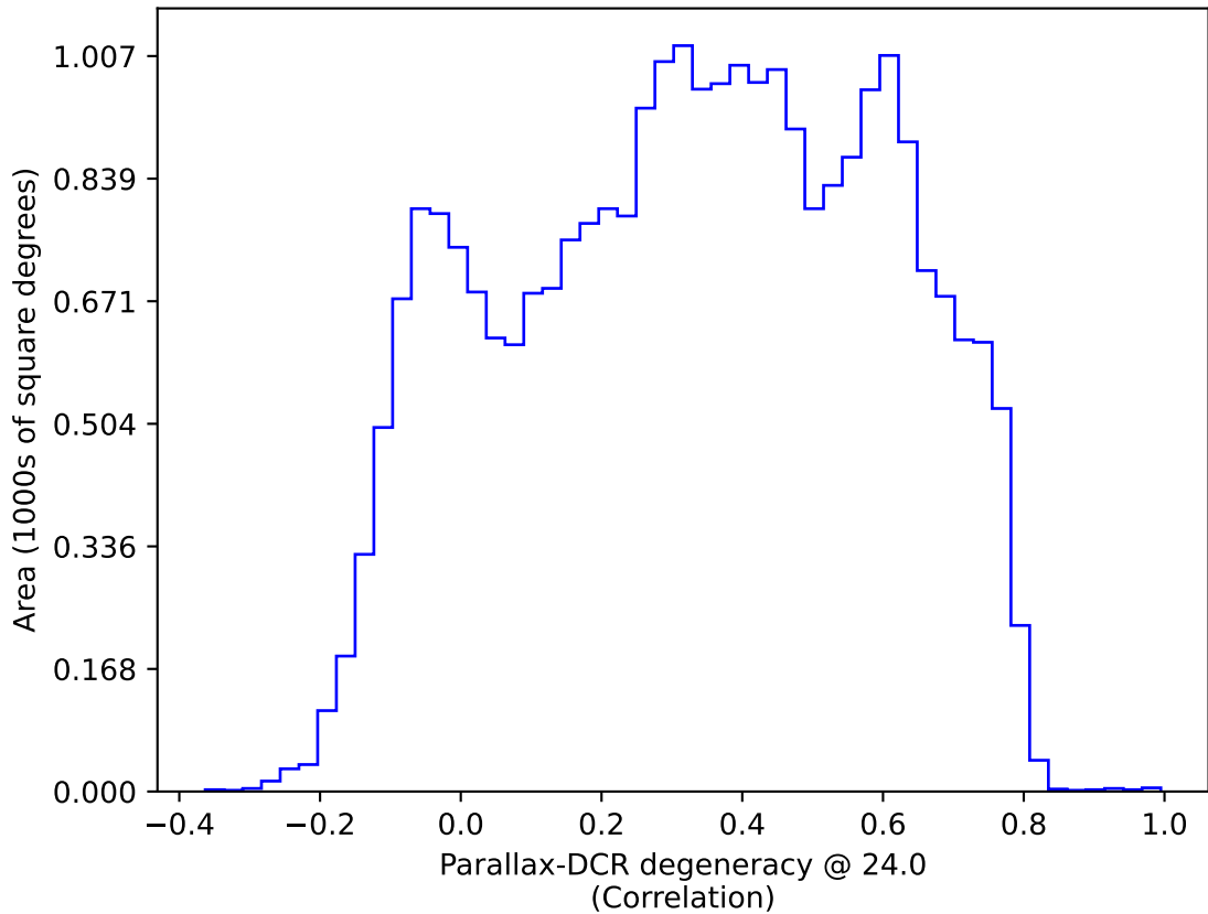
ddf_loaded_fl8_v3.4_10yrs All sky: Parallax-DCR degeneracy @ 24.0
