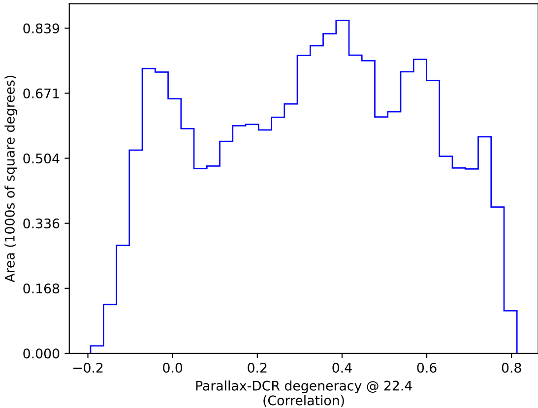
ddf_loaded_fl8_v3.4_10yrs WFD: Parallax-DCR degeneracy @ 22.4
