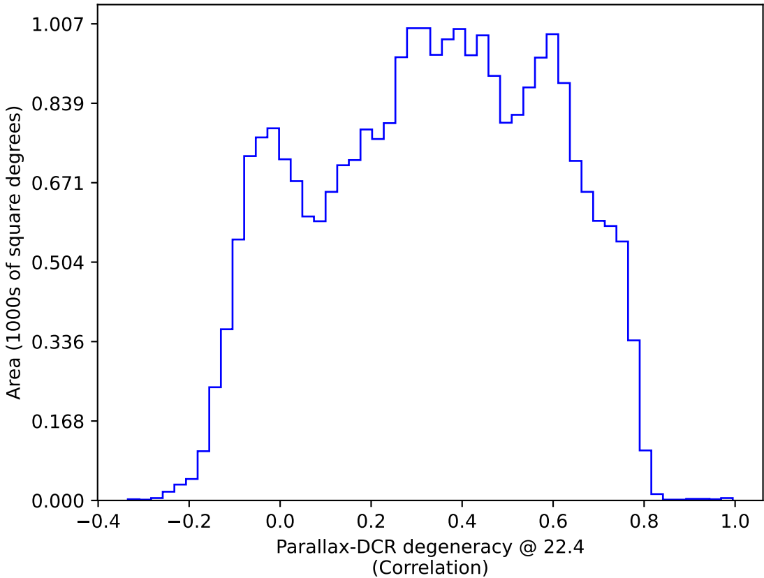
ddf_loaded_fl8_v3.4_10yrs All sky: Parallax-DCR degeneracy @ 22.4
