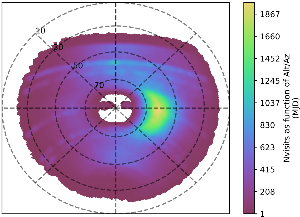
ddf_loaded_fl8_v3.4_10yrs y band: Nvisits as function of Alt/Az
