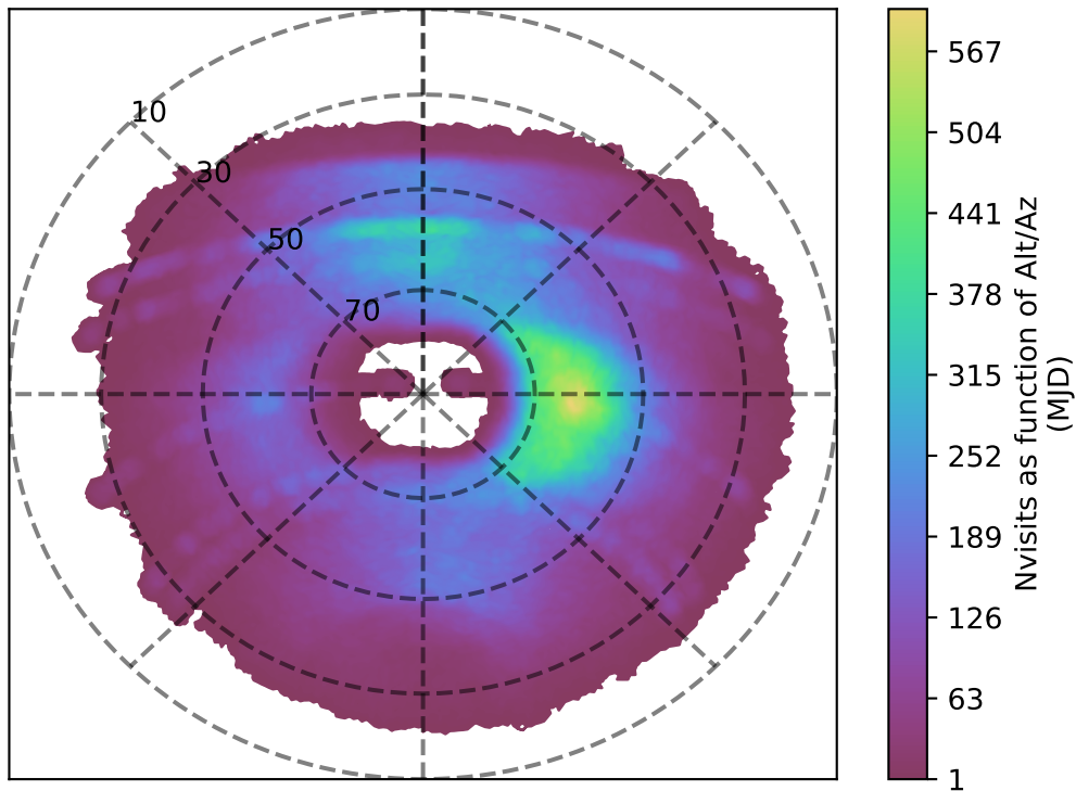
ddf_loaded_fl8_v3.4_10yrs u band: Nvisits as function of Alt/Az
