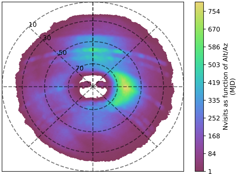
ddf_loaded_fl8_v3.4_10yrs g band: Nvisits as function of Alt/Az
