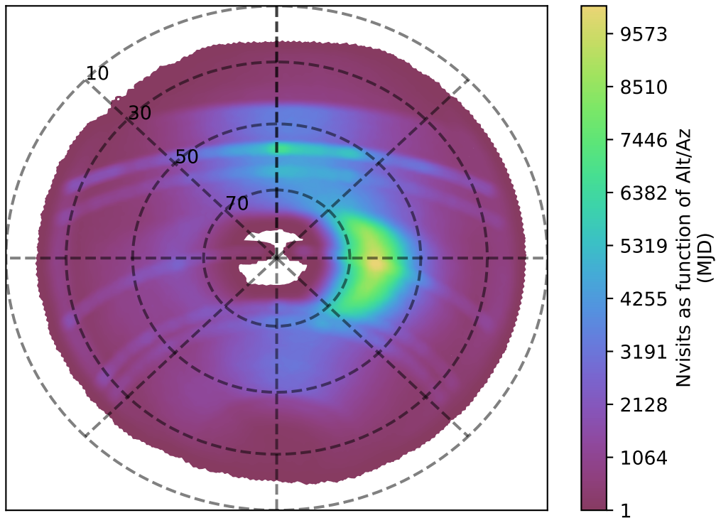
ddf_loaded_fl8_v3.4_10yrs all bands: Nvisits as function of Alt/Az
