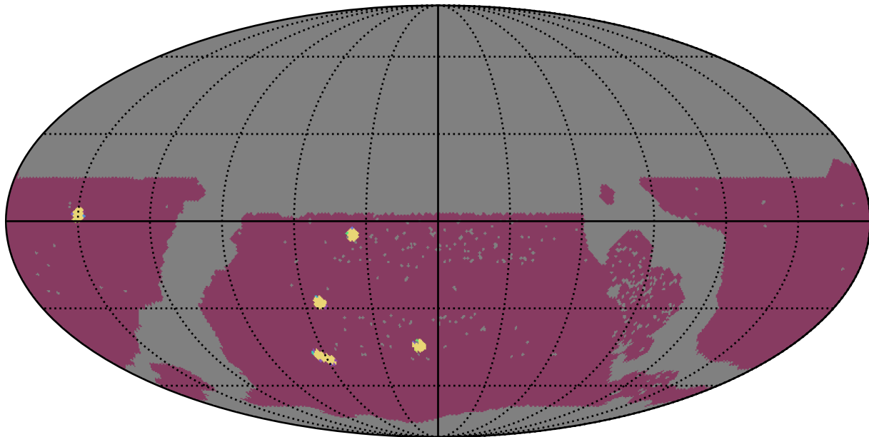
ddf_loaded_fl8_v3.4_10yrs WFD: NumberOfQuickRevisits
