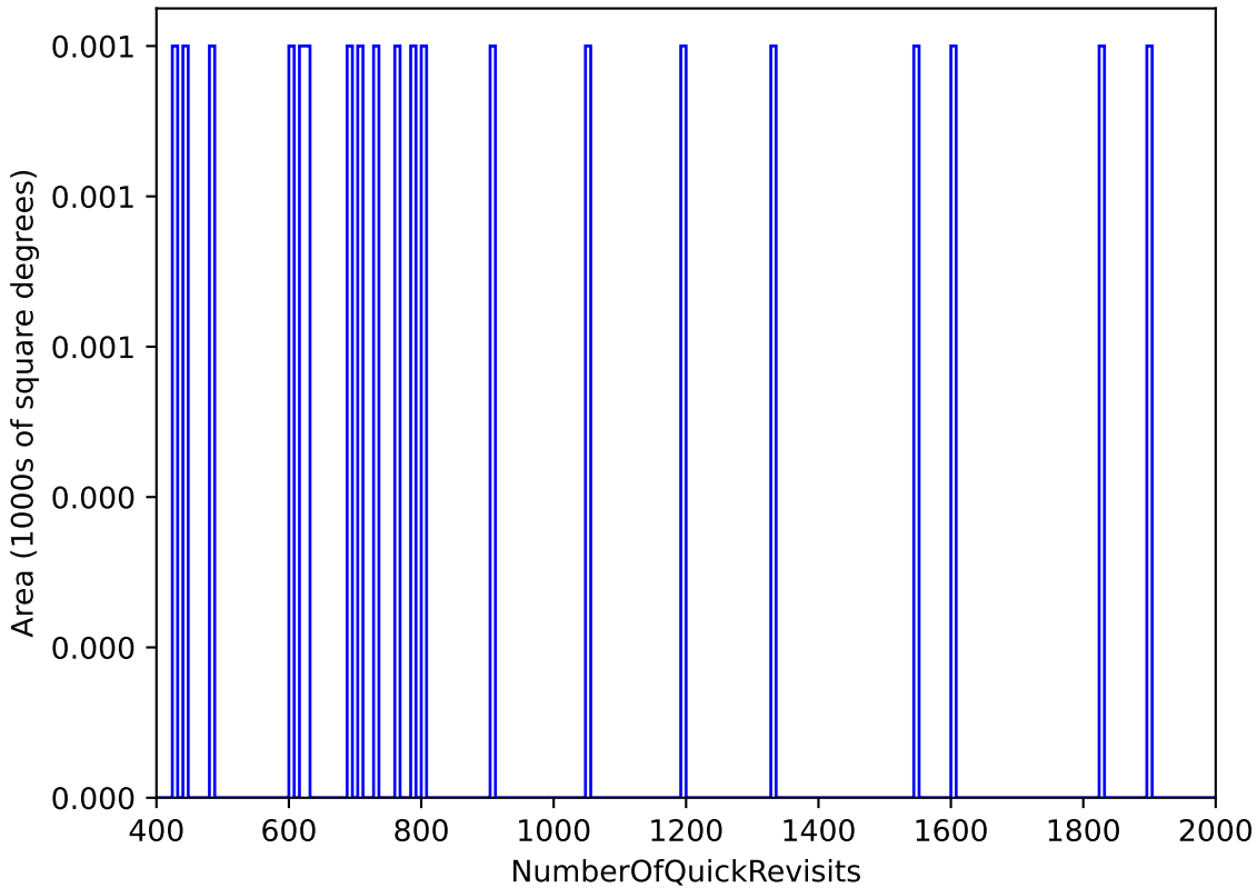
ddf_loaded_fl8_v3.4_10yrs WFD: NumberOfQuickRevisits
