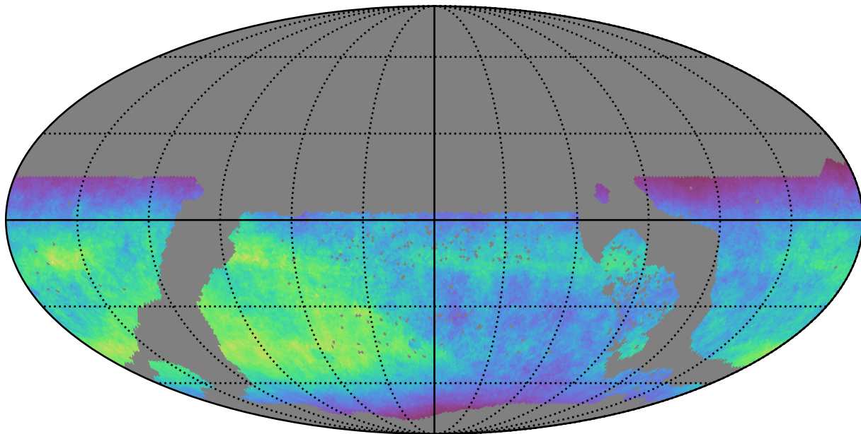
ddf_loaded_fl8_v3.4_10yrs WFD z band: Normalized Teff
