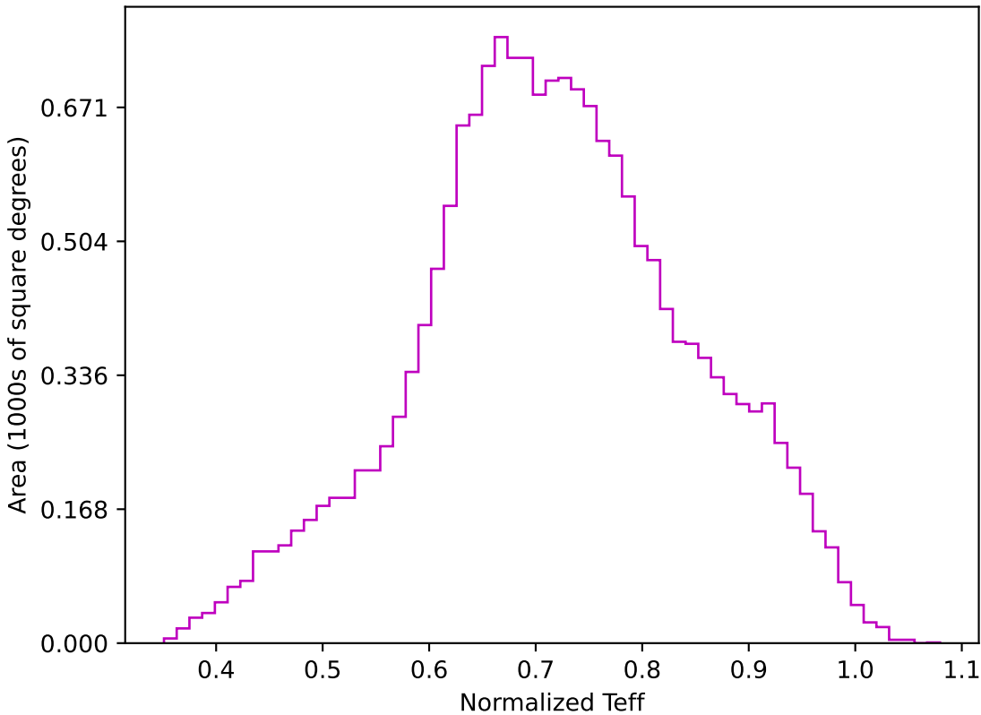
ddf_loaded_fl8_v3.4_10yrs WFD z band: Normalized Teff
