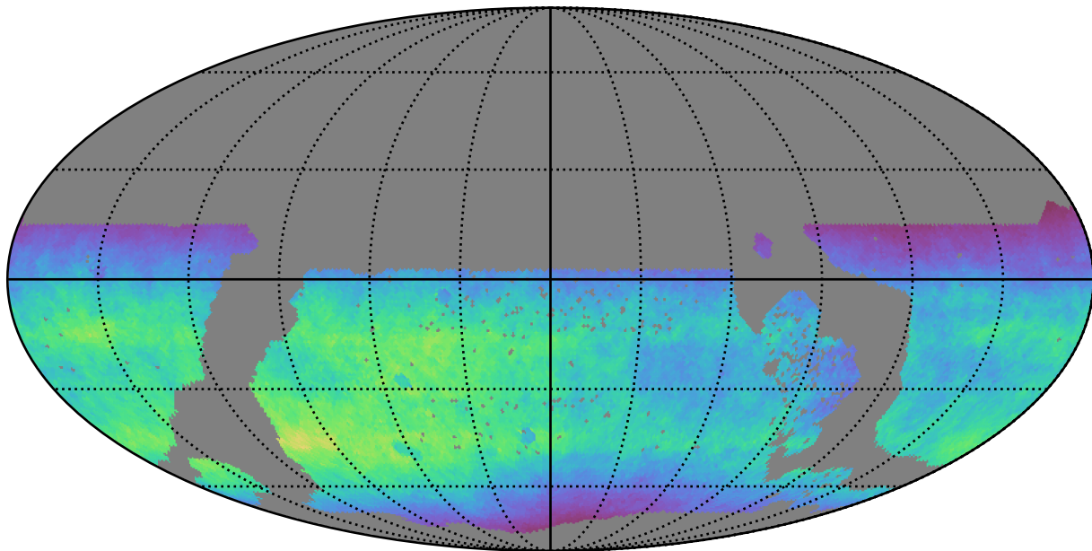
ddf_loaded_fl8_v3.4_10yrs WFD y band: Normalized Teff
