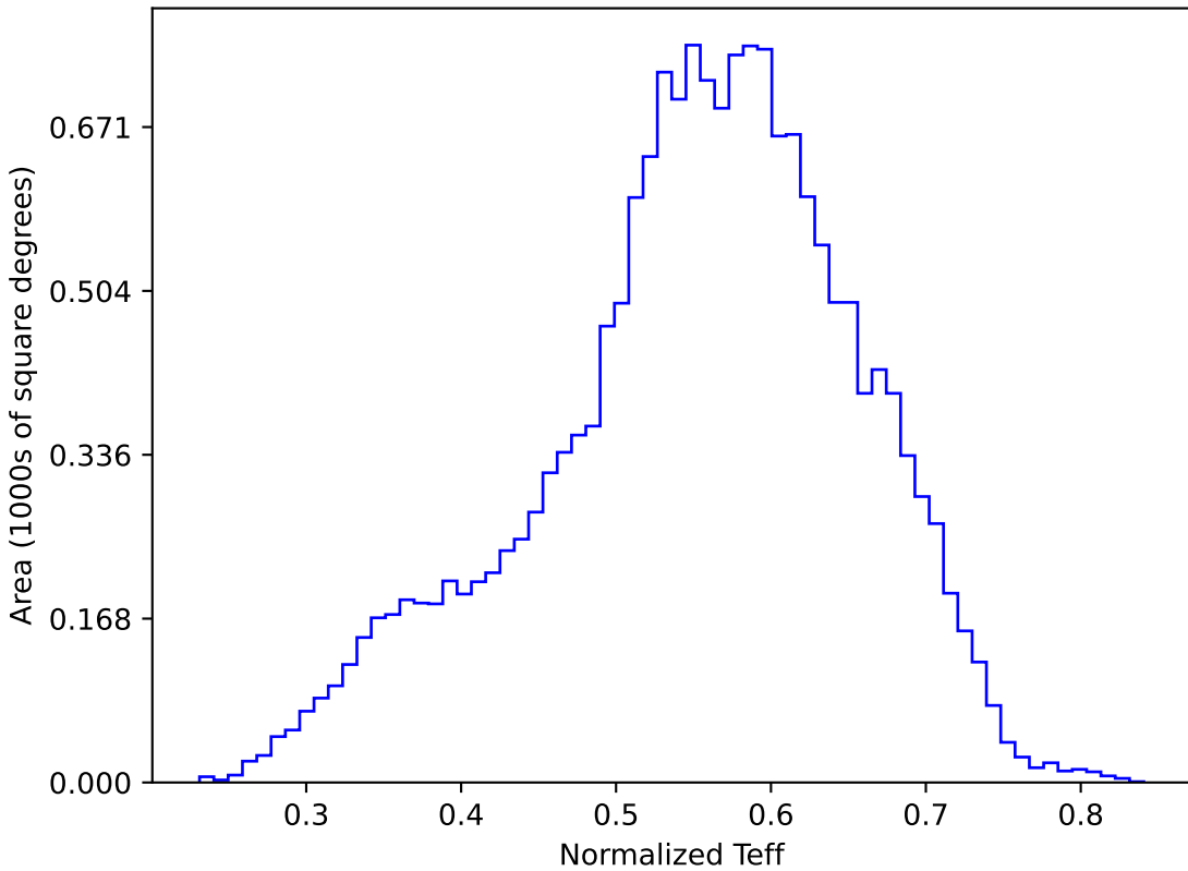
ddf_loaded_fl8_v3.4_10yrs WFD y band: Normalized Teff
