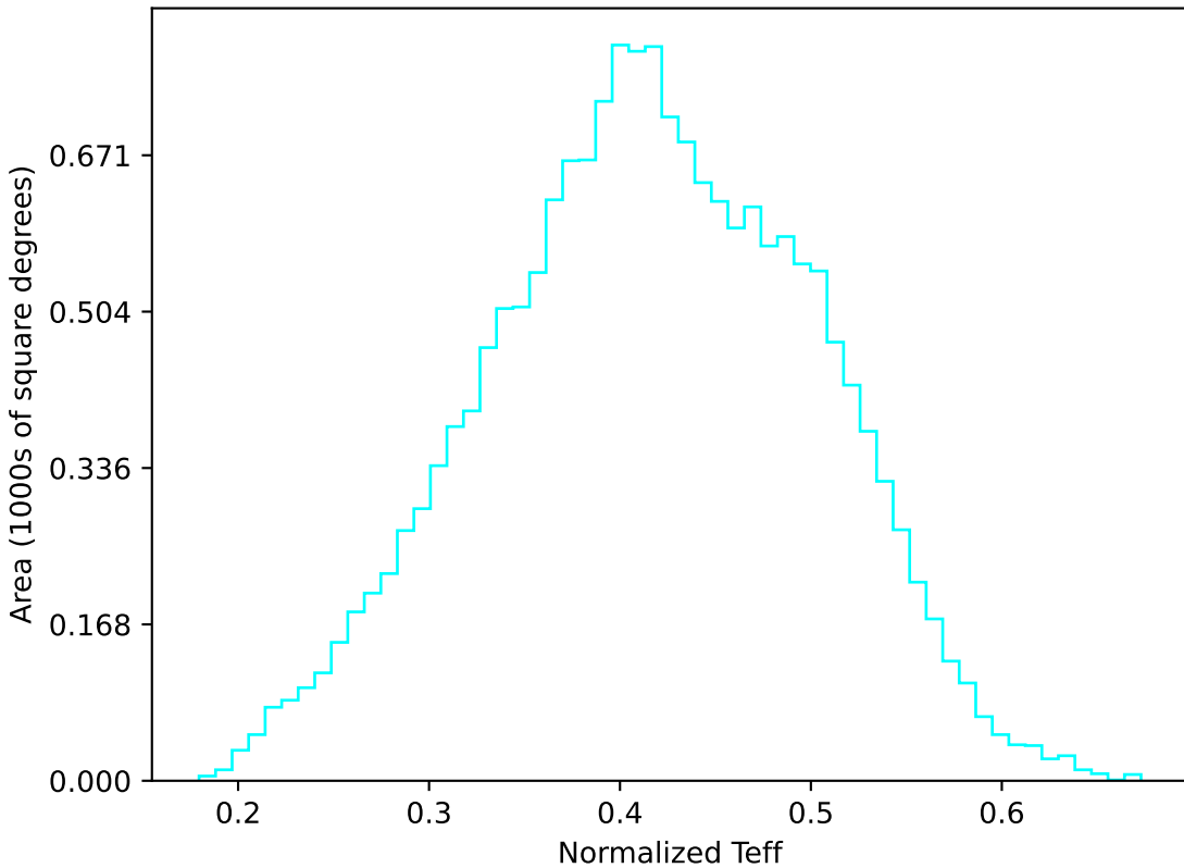
ddf_loaded_fl8_v3.4_10yrs WFD u band: Normalized Teff
