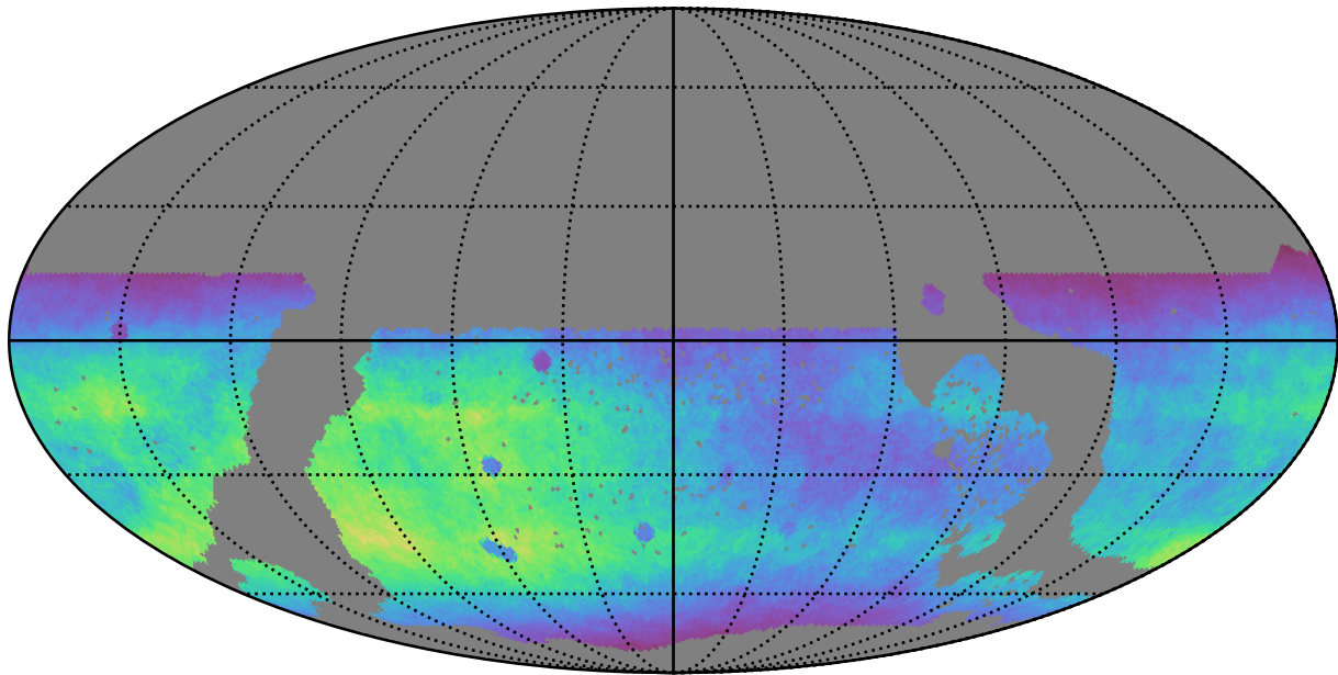
ddf_loaded_fl8_v3.4_10yrs WFD r band: Normalized Teff
