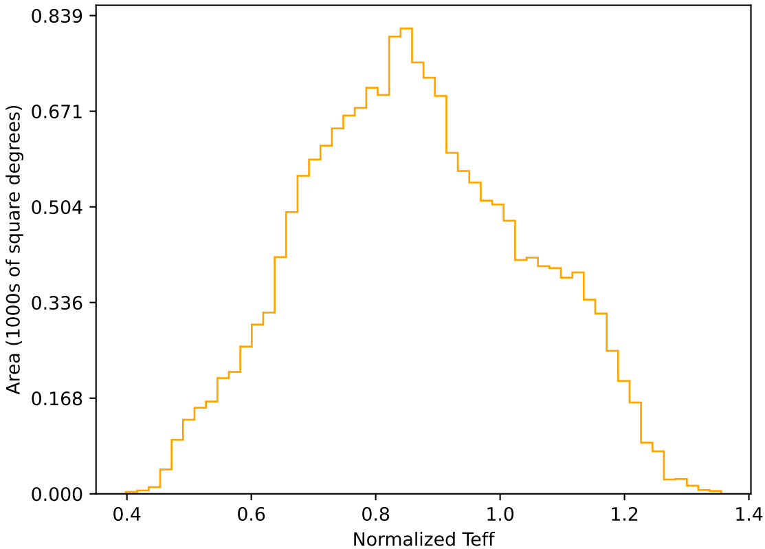
ddf_loaded_fl8_v3.4_10yrs WFD r band: Normalized Teff
